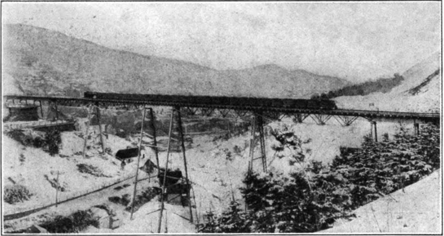
COMPRESSED AIR MOTOR CAR HAULING 28 STEEL BOTTOM-DUMPING CARS, CONTAINING 4 TONS OF ORE EACH FROM ELLISON HOIST TO MILLS OF HOMESTAKE MINING COMPANY, OVER STEEL BRIDGE, 100 FEET HIGH.
