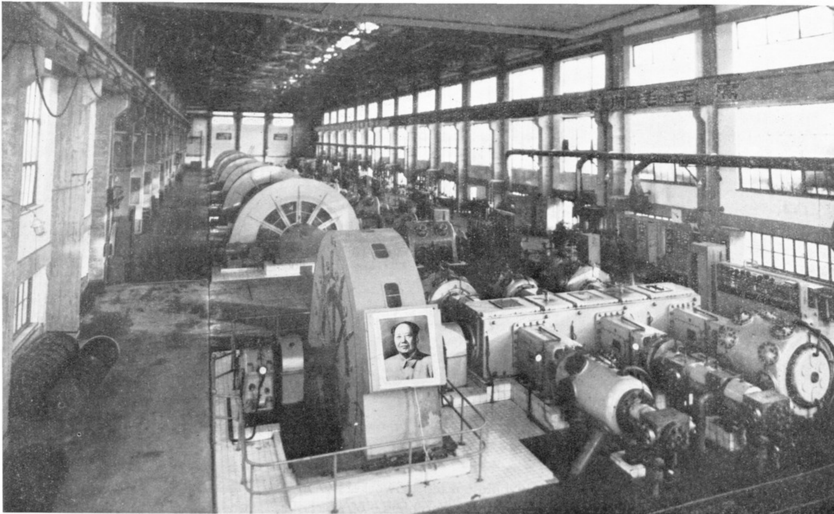
The symmetric balanced compressor made in China.
